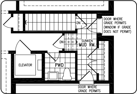
OPT. ELEVATOR ELEVATION C
