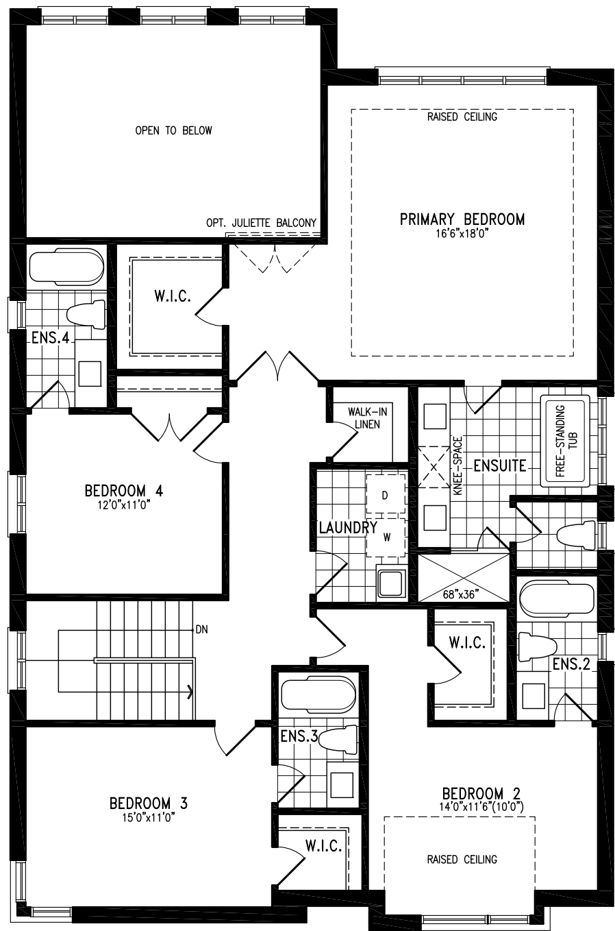
SECOND FLOOR ELEVATION C OPT. LAUNDRY
